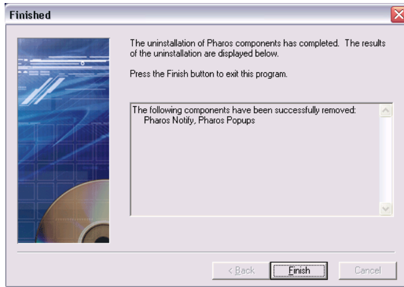
Figure 7: Pharos Uninstaller
