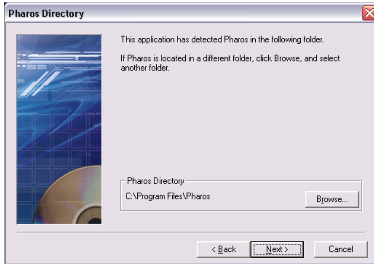
Figure 5: Pharos Uninstaller
