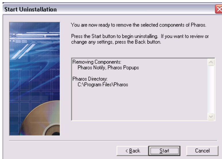
Figure 6: Pharos Uninstaller
