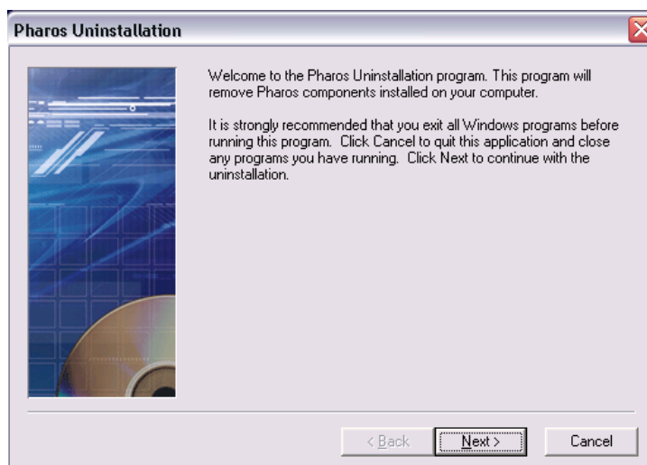
Figure 3: Pharos Uninstaller
