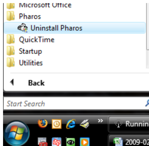
Figure 1: Start Menu
