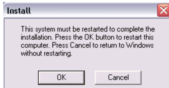
Figure 8: Pharos Uninstaller
