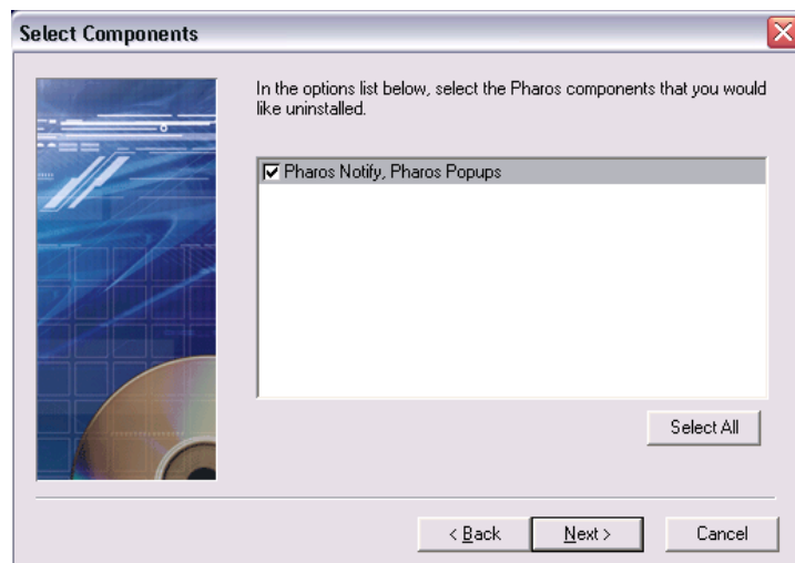
Figure 4: Pharos Uninstaller
